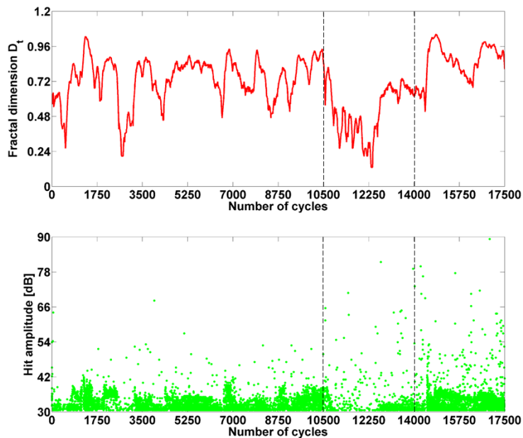
Fig. 6. Type 1 notched specimen, fractal dimension D_t of the registered hits over time above and their representation as green dots in a Amplitude vs Time diagram below.
