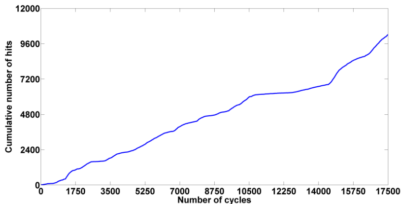
Fig. 4. Cumulative number of hits vs number of cycles for the type 1 notched specimen.
