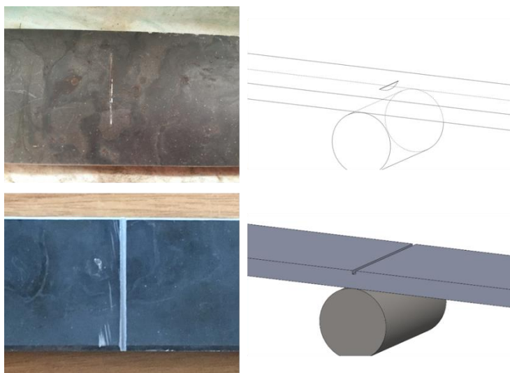
Fig. 2. Details of the considered notches with their CAD representations: type 1 above and type 2 below.
